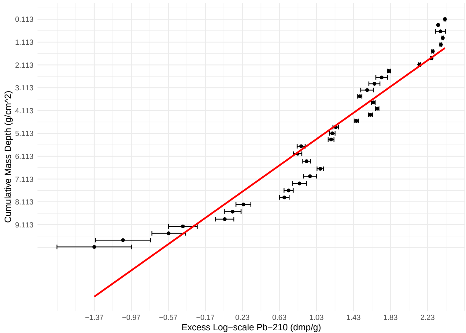
Excess Log-scale Pb-210 vs Cumulative Mass Depth
